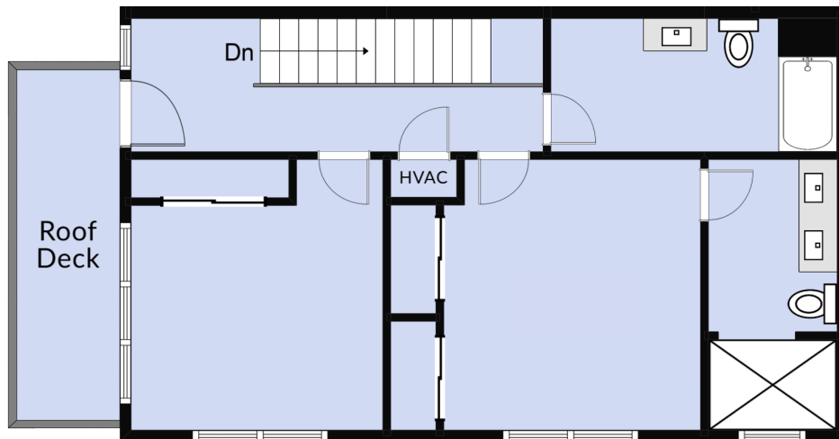
UPPER LEVEL
